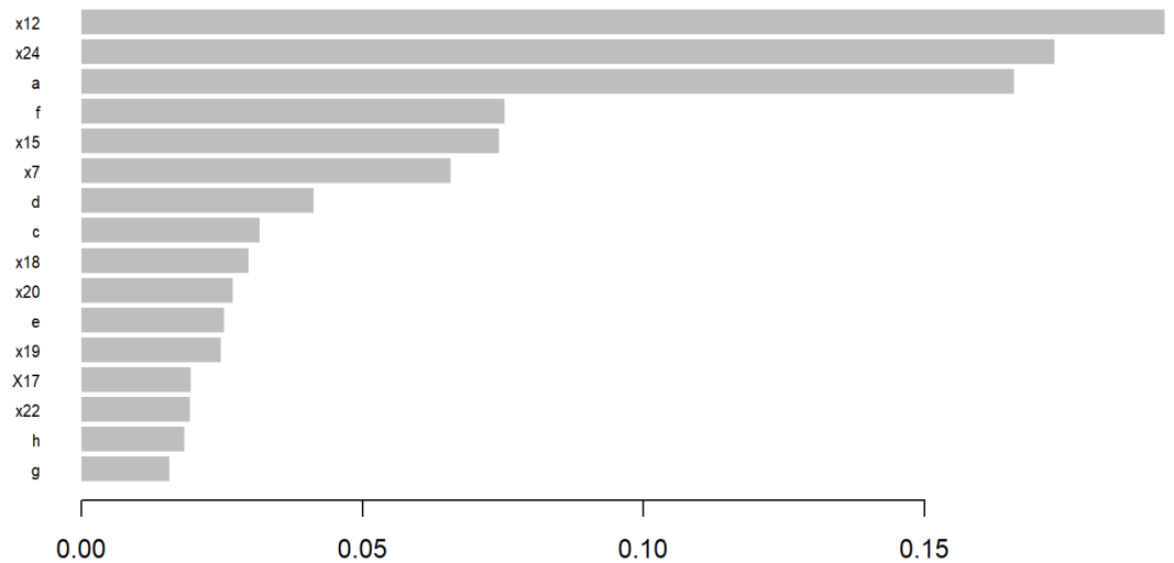
Figure 2: Feature Importance Plot of XGBOOST Regression.
