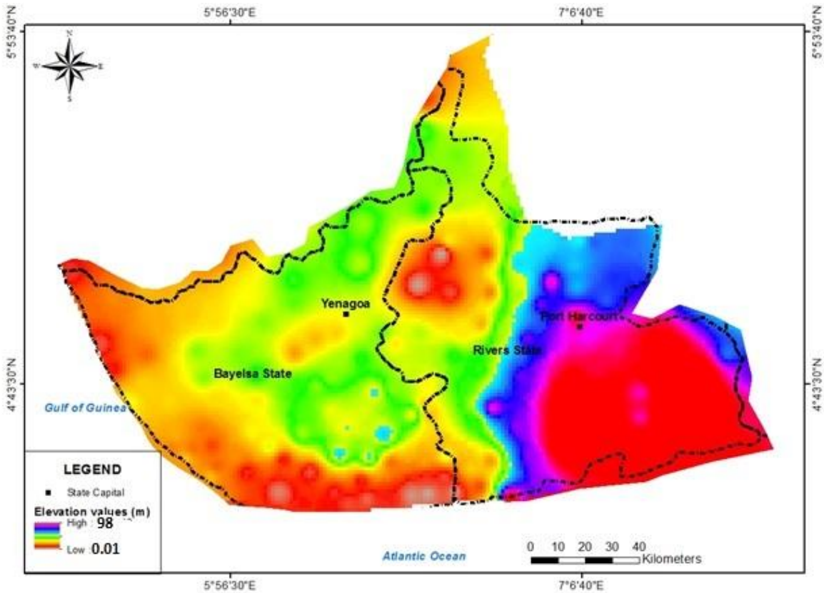
Figure 2: Digital terrain map of the study area
