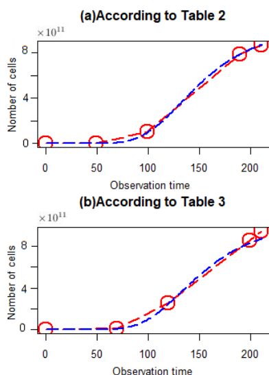
Fig. 2. Comparison of the tumor cell dynamics
