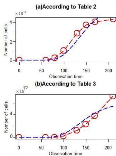
Fig. 6. Dormant cells dynamics (red) and its estimated (blue)
