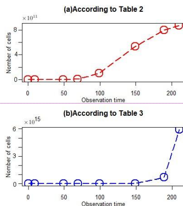
Fig. 5. Resistant cells dynamics.
