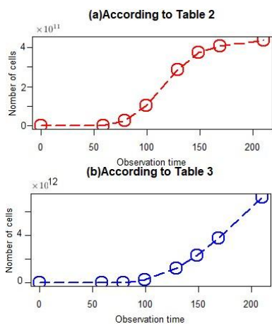
Fig. 4. Dormant cells dynamics.
