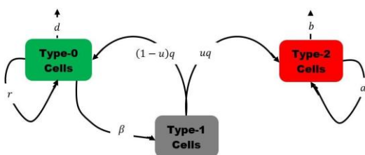
Fig. 1. Interaction schematics of dormant cancer tumor cells.
