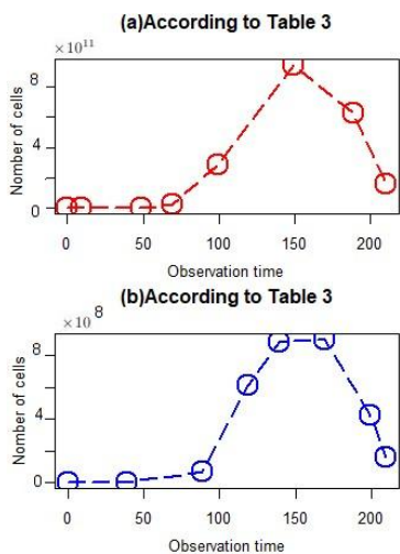
Fig. 3. Susceptible cells dynamics.
