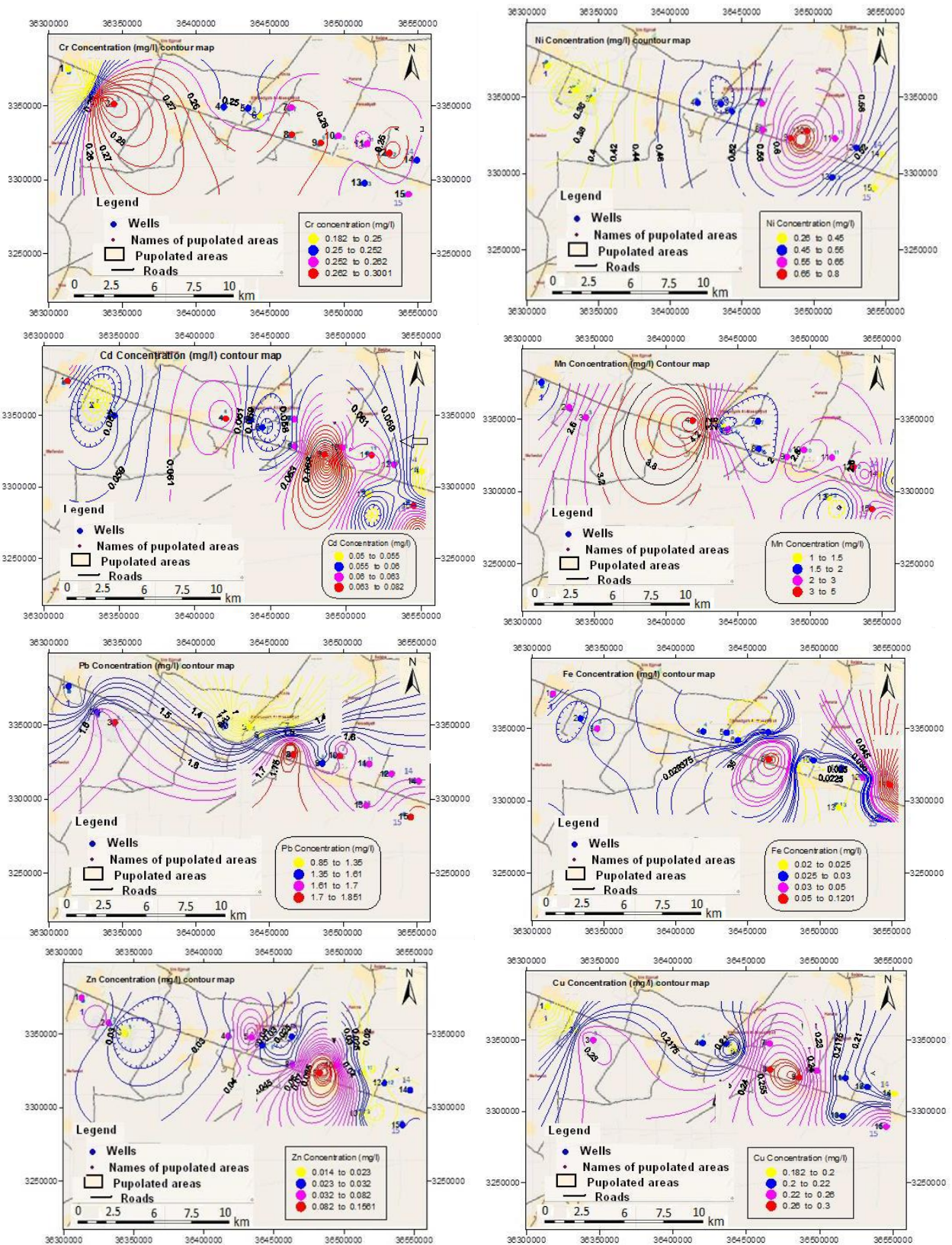
Figure(4):Contourmapshowstheconcentration(mg/l)ofCr,Ni,Cd,Mn,Pb,Fe,ZnandCu for the study water well samples.
