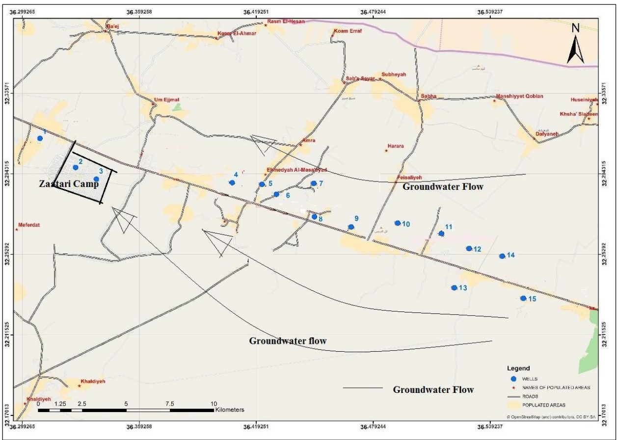
Figure(2):Locationmapofthecollected waterwellsamplesanddirectionofgroundwater flow.
