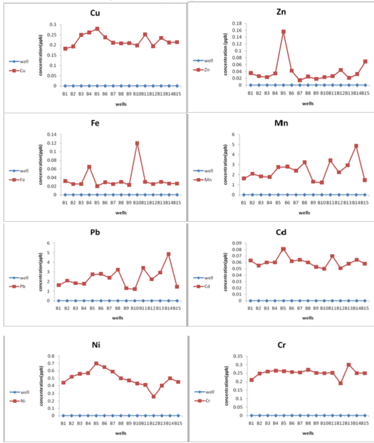
Figure(3):Concentration(ppb)fortheelementsCu,Zn,Fe,Mn,Pb,Cd,NiandCrinthestudy water well samples.
