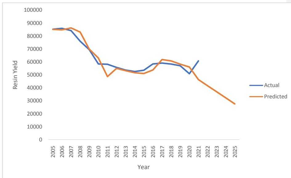
Fig 2: Actual and predicted values of resin yield by using a single exponential smoothing model.
