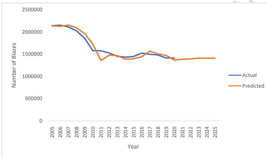
Fig 1: Actual and predicted values of the number of blazes by using a single exponential smoothing model
