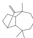
(e) longifolene
