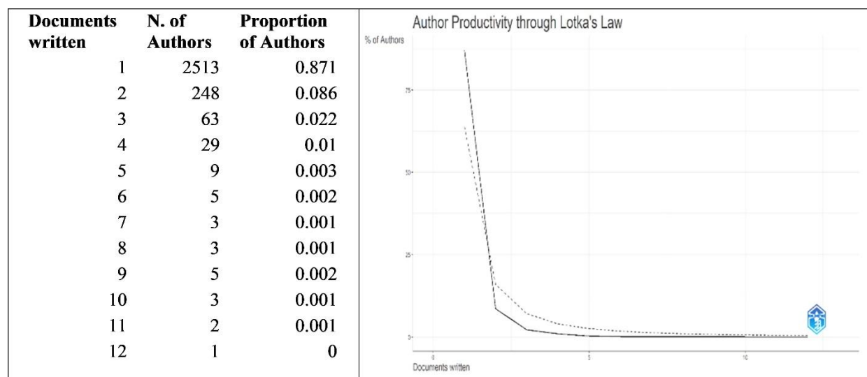
Fig 6: Lotka's Law
