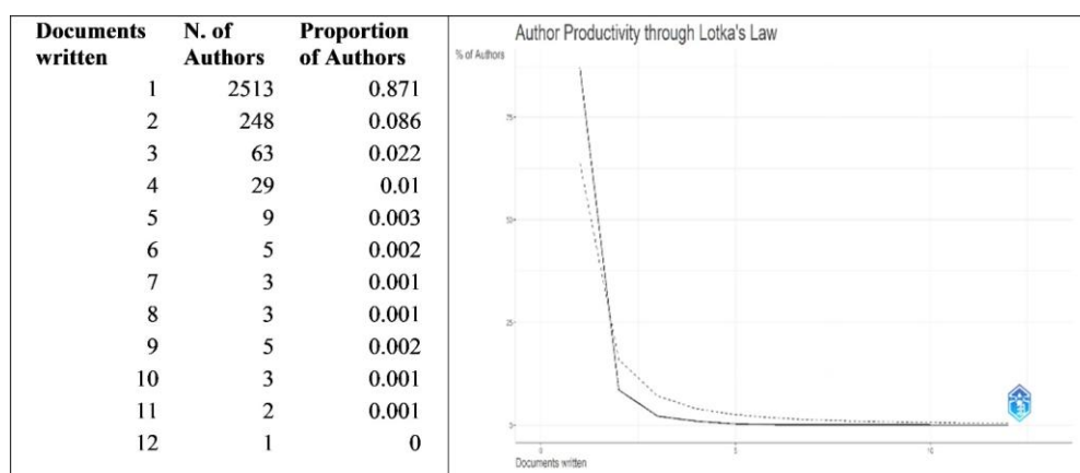
Fig 6: Lotka's Law
