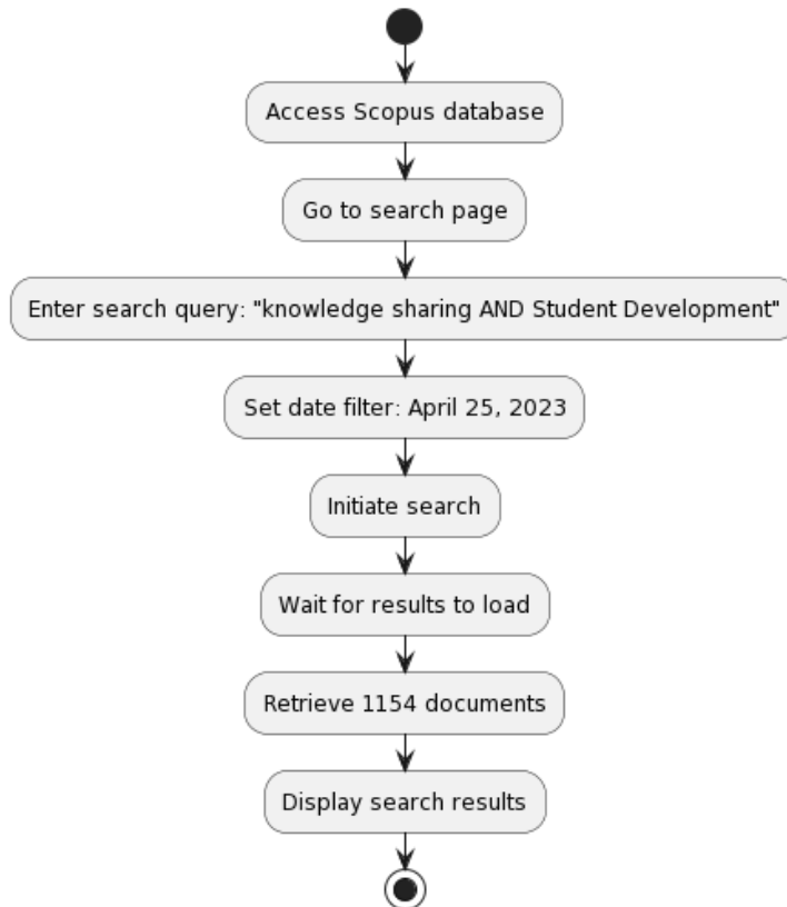
Fig 1: Search process
