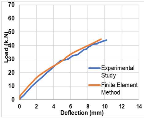
g) Load-Deflection Curves for Beam (G2).
