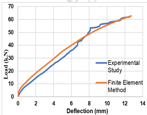
k) Load-Deflection Curves for Beam (F3).
