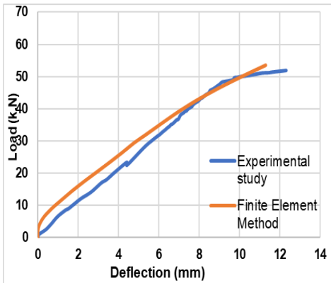
i) Load-Deflection Curves for Beam (F1).
