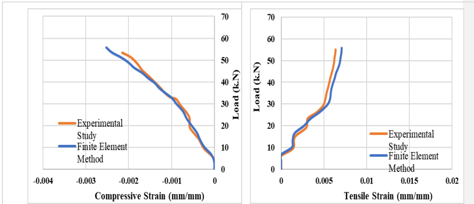
j) Load-Compressive and Tensile Strain Curves for Beam (F2).
