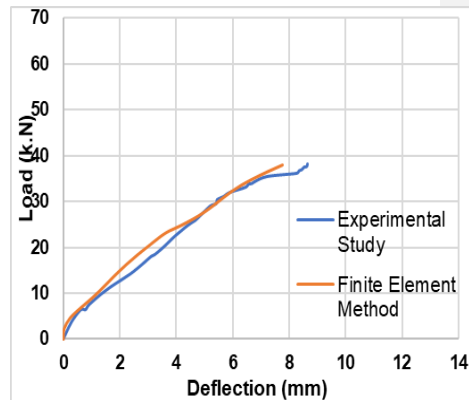
f) Load-Deflection Curves for Beam (G1).
