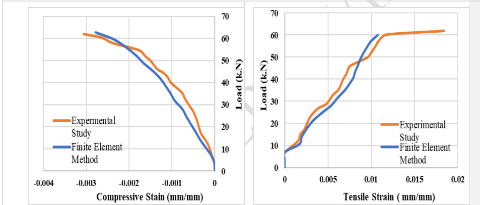
k) Load-Compressive and Tensile Strain Curves for Beam (F3).
