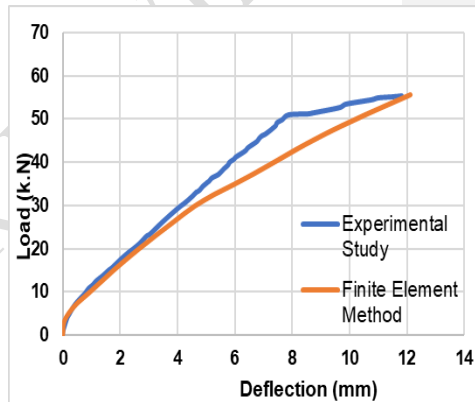
j) Load-Deflection Curves for Beam (F2).
