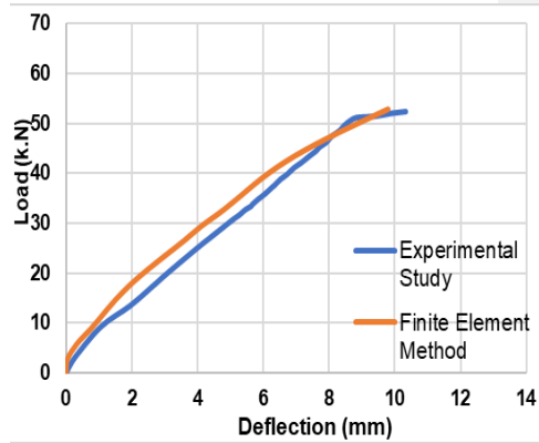
h) Load-Deflection Curves for Beam (G3).
