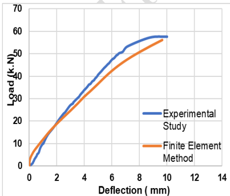
e) Load-Deflection Curves for Beam (B3).
