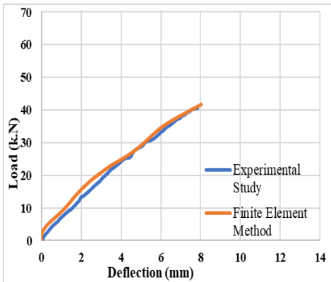
c) Load-Deflection Curves for Beam (B1).
