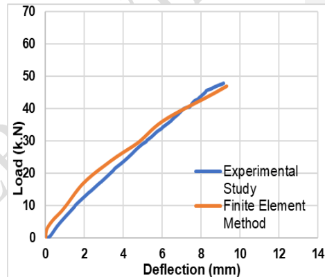
d) Load-Deflection Curves for Beam (B2).
