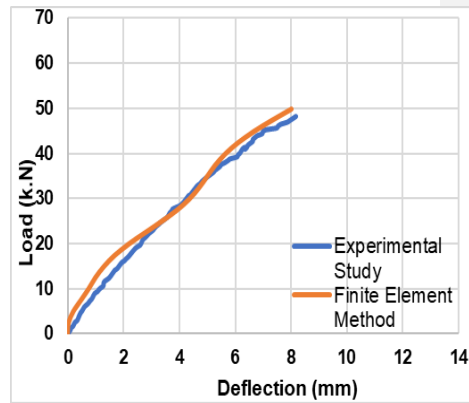
b) Load-Deflection Curves for Beam (A2).
