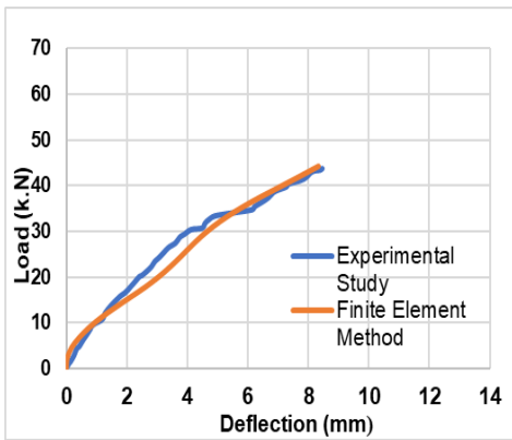
a) Load-Deflection Curves for Beam (A1).
