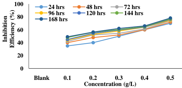
Figure 2: Inhibition Efficiency against CBL Inhibitor Concentration at Room Temperature (30±2).
