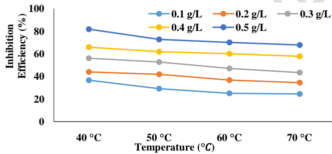
Figure4: Variation of Inhibition Efficiency of CBL Extract with different Concentrations and Temperatures after 3 hours of Immersion
