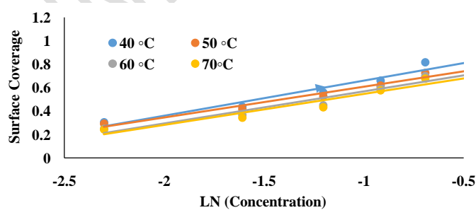
Figure 6: Langmuir Adsorption Isotherm for Mild Steel in 1 M HCl Solution in the Presence of CBL Extract.
