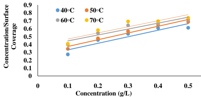
Figure 6: Langmuir Adsorption Isotherm for Mild Steel in 1 M HCl Solution in the Presence of CBL Extract.
