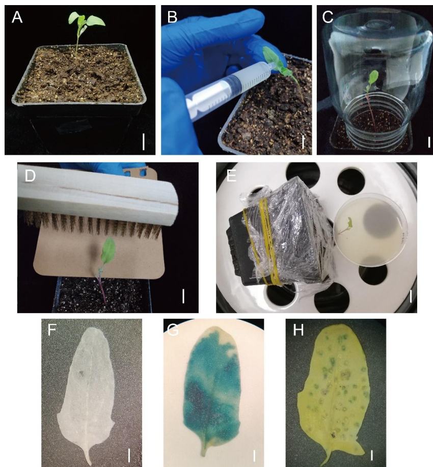
Figure 4 Agroinfiltration of quinoa leaves. Leaf was used for agroinfiltration from 5-day-old seedling (A), leaf was injected at the abaxial side with a needleless syringe (B), the treated seedlings were covered with a plastic jar for recovery for 4 days (C), leaf was pressed at the abaxial side by the brush (D), leaf was incubated in Agrobacterium culture and vacuumed at 0.7 MPa for 1 min (E), the GUS staining of leaf injected with 1/10 MS culture (CK) (F), GUS assay of leaf injection (G), GUS assay of leaf vacuum penetration (H). Scale bar A-E: 1cm; F-H: 0.2 cm.
