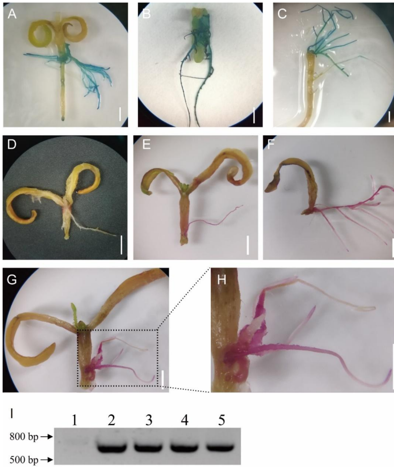
Figure 2 GUS assay with hairy hoots from three types of explants: CHE (A), CE (B), HE (C), GUS assay with hairy roots from the negative control (D); red pigmentation in hairy roots: CHE (E), CE (F), CHE (G) and details of hairy roots with enlarged scale (H); PCR analysis of GUS gene: 1 DNA from original roots as a negative control, 2 plasmid of PTF102 as a positive control, 3-5 DNA from hairy roots of CHE, CE, HE (I). Scale bar A-C: 0.2 cm, D-H: 0.25 cm.
