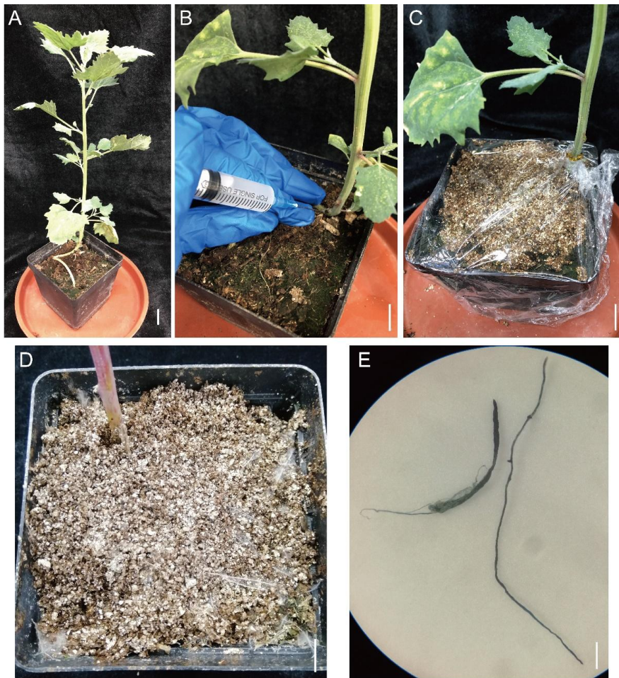
Figure 3 Hairy roots induction in-vivo . 2-month-old seedling was used for injection (A), the taproot was injected with a syringe needle (B), covered with wet vermiculite and plastic film to keep humid (C), hairy roots of quinoa injection hairy roots grew out from quinoa's tap root after two weeks(D), hairy roots cut from the tap root and assay for \beta -glucuronidase activity (E). Scale bar A:0.5 cm; B-C:1 cm; D-E:0.25 cm.
