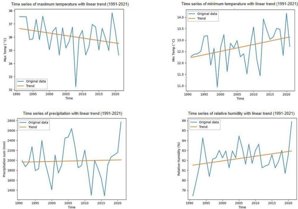
Figure 2: Time series plots with the linear trend for the variables maximum temperature, minimum temperature, precipitation, and relative humidity for a period of 30 years (1991-2021).
