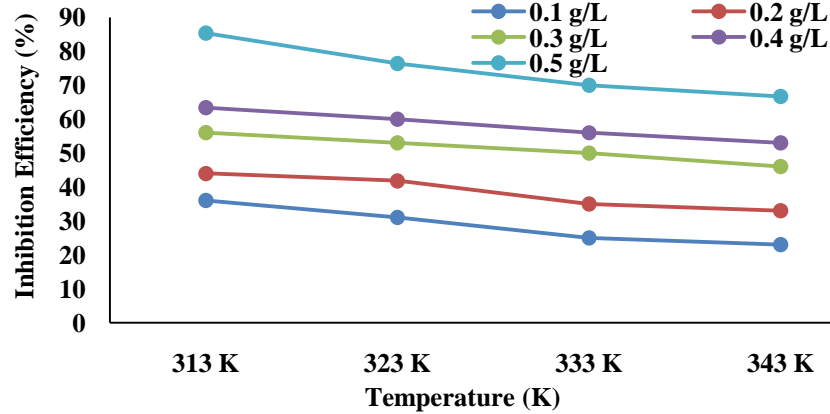
Fig. 5. Variation of inhibition efficiency of AHL inhibitor with temperature at various concentrations
