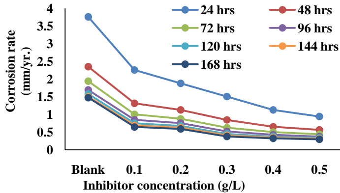
Fig. 2. Corrosion Rate against AHL Inhibitor Concentration in 1 M HCl Solution
