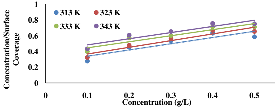
Fig. 7. Langmuir adsorption isotherm for mild steel in 1 M HCl solution in the presence of AHL extract
