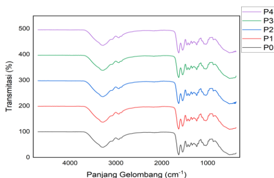
Figure 1. Wavelength (Functional Group) of FTIR
