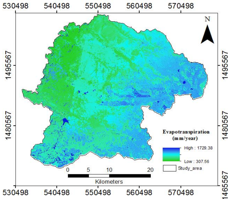
Figure 2. Annual actual evapotranspiration grid map of the study area
