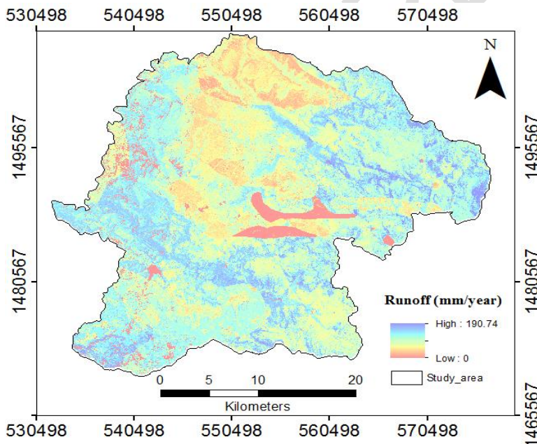
Figure 3. Annual surface runoff grid map of Mekelle area
