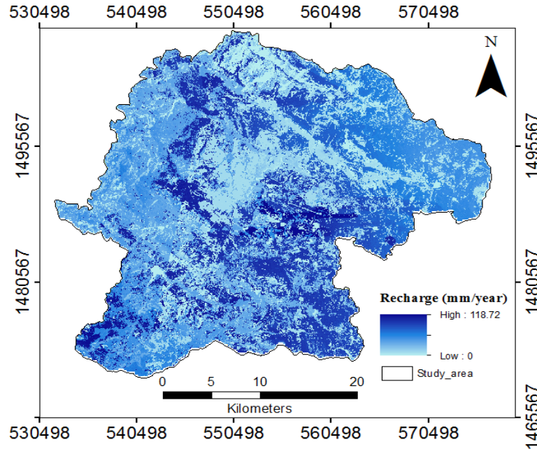
Figure 4. Annual groundwater recharge grid map of Mekelle area.
