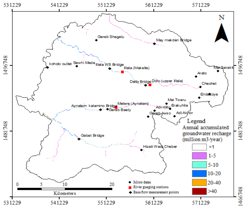
Figure 6. Accumulated annual groundwater recharge grid maps in the study area
