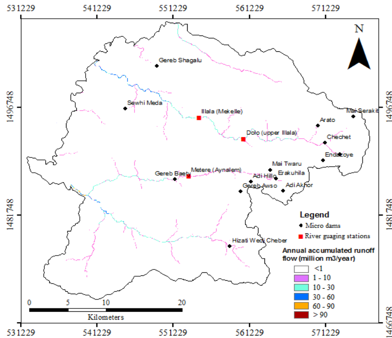
Figure 5. Accumulated annual flow (Surface runoff plus groundwater recharge) grid maps of the study area.
