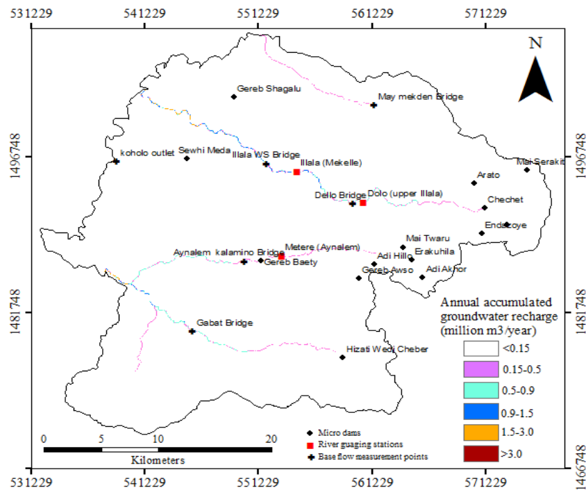
Figure 7. Accumulated winter groundwater recharge grid maps in the study area
