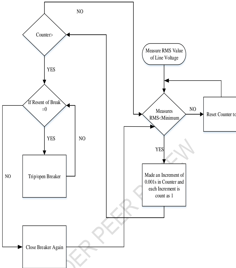
Fig. 3. Dynamical operation of under voltage relay
