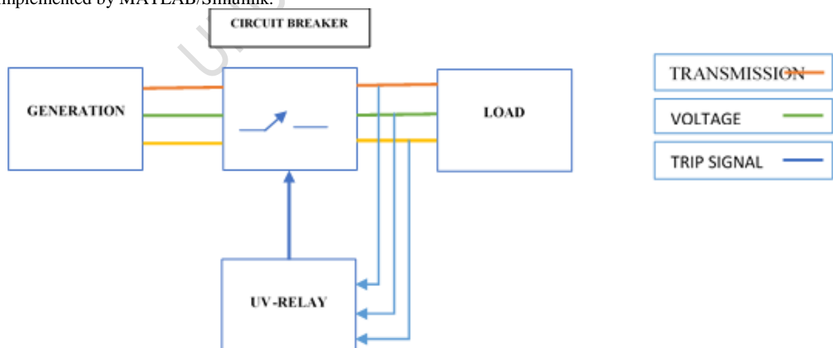
Fig. 1. Block diagram of the protected system
