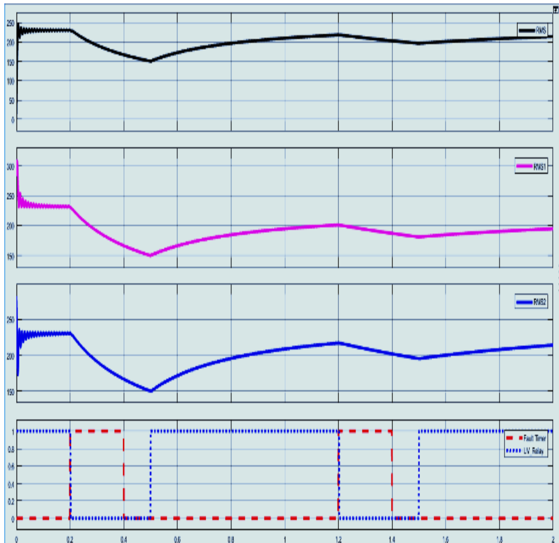
Fig. 5. Turn-ON three-phase to ground faults in phases A, B, and C.
