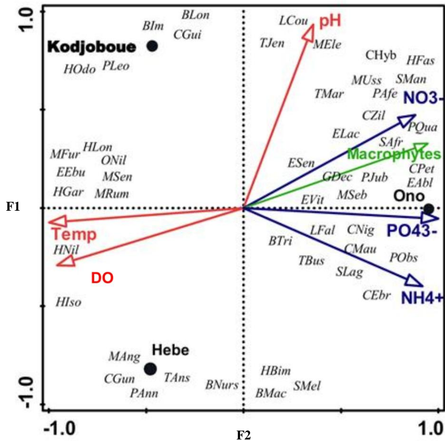
Figure 2: Graphical representation of Canonical redundancy analysis based on the abundance of 50 fish species, environmental variables (Temp = water temperature, DO = dissolved oxygen, pH, NO 3 - = nitrate, PO 4 3- = phosphate and NH 4 + = ammonium-nitrogen), and lagoons (geometric figures) during the period-September 2015 to August 2016.
