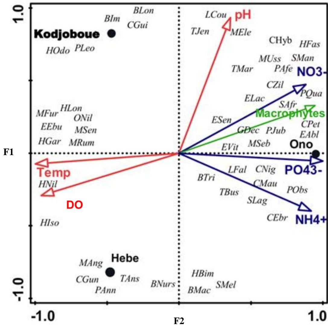
Figure 2: Graphical representation of Canonical redundancy analysis based on the abundance fish assemblage of 50 fish species, environmental variables (Temp = water temperature, DO = dissolved oxygen, pH, \text{NO}_3^- = nitrate, \text{PO}_4^{3-} = phosphate and \text{NH}_4^+ = ammonium-nitrogen), and lagoons (geometric figures) during the period-September 2015 to August 2016.
