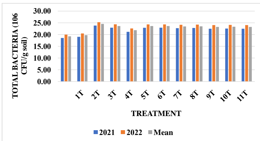
Fig.5- Effect of application of Nano-DAP fertilizer on total bacteria in soil 60 DAT in rice during 2021 and 2022 (x 10 6 CFU g -1 ).
