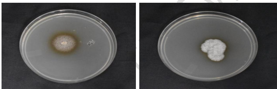
Plate 2. Lignin Degrading Fungi
