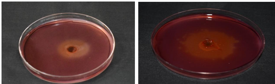
Plate 1. Cellulose Degrading Bacteria
