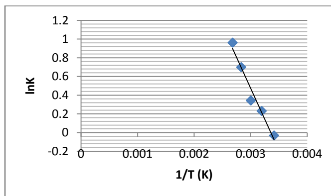
Fig 11: Thermodynamic plot of Pb(II) onto SSM
