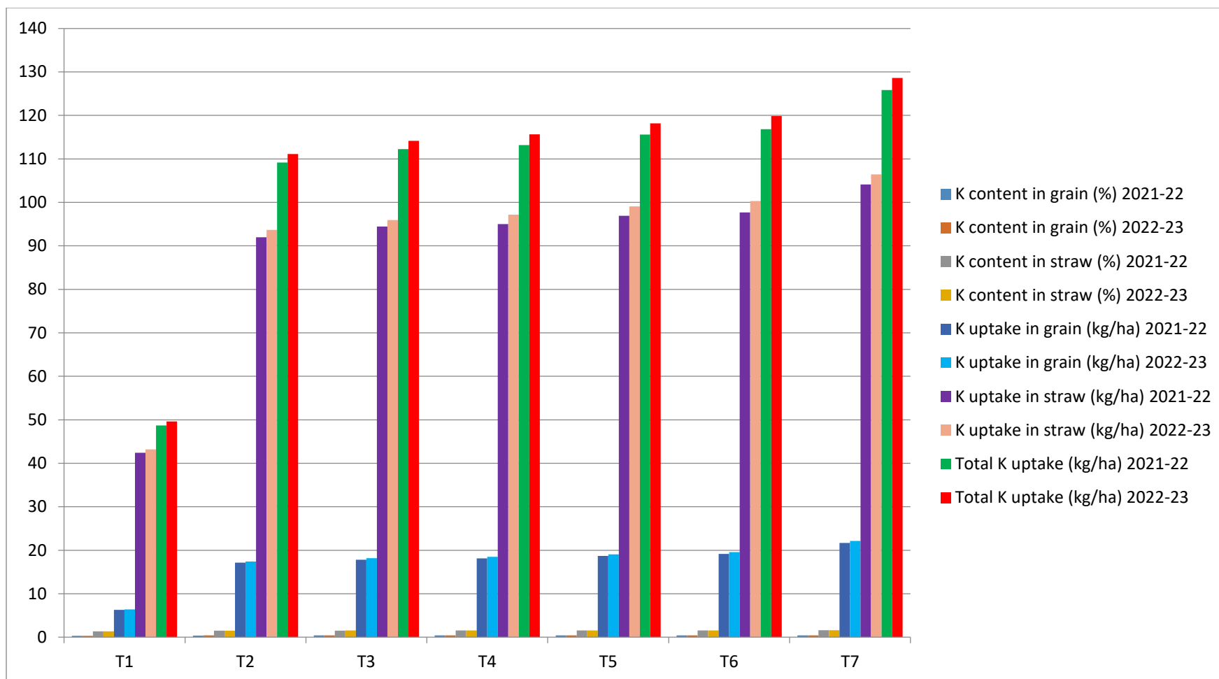
Fig. 3 Effect of different nutrient management approaches on K content (%), K uptake and Total K uptake ( \text{kg ha}^{-1} ) in grain and straw of wheat
