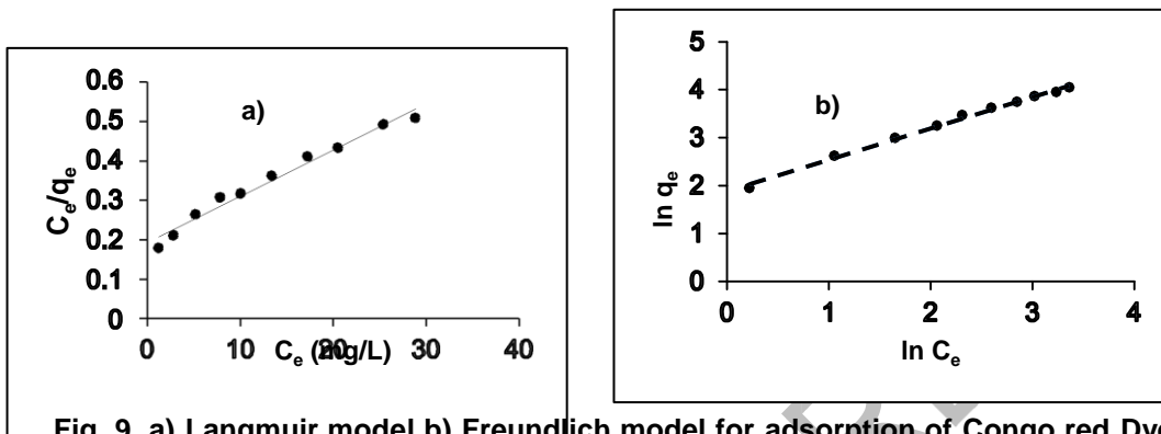
Fig. 9. a) Langmuir model b) Freundlich model for adsorption of Congo red Dye onto CuO nanoparticles
