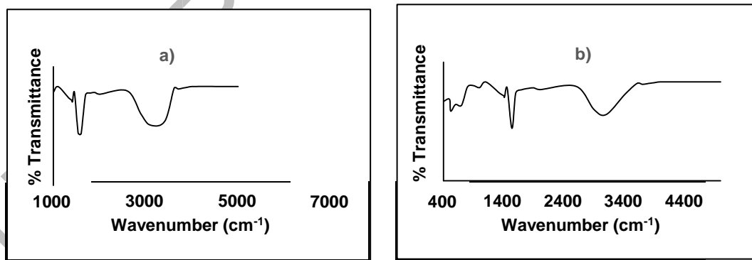
Fig. 2. a) FTIR spectrum of Ficus benghalensis b) FTIR spectrum of Ficus benghalensis assisted CuO nanoparticles
