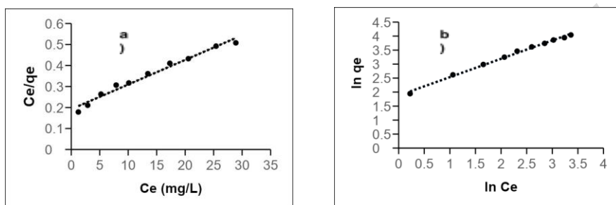
Fig. 9. a) Langmuir model b) Freundlich model for adsorption of Congo red Dye onto CuO nanoparticles
