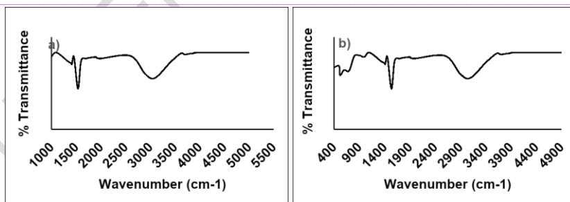
Fig. 3. a) FTIR spectrum of Ficus benghalensis b) FTIR spectrum of Ficus benghalensis assisted CuO nanoparticles
