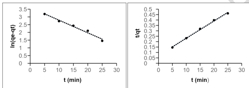
Fig. 8. a) Pseudo first order b) second order kinetic models for adsorption of Congo red dye onto CuO nanoparticles
