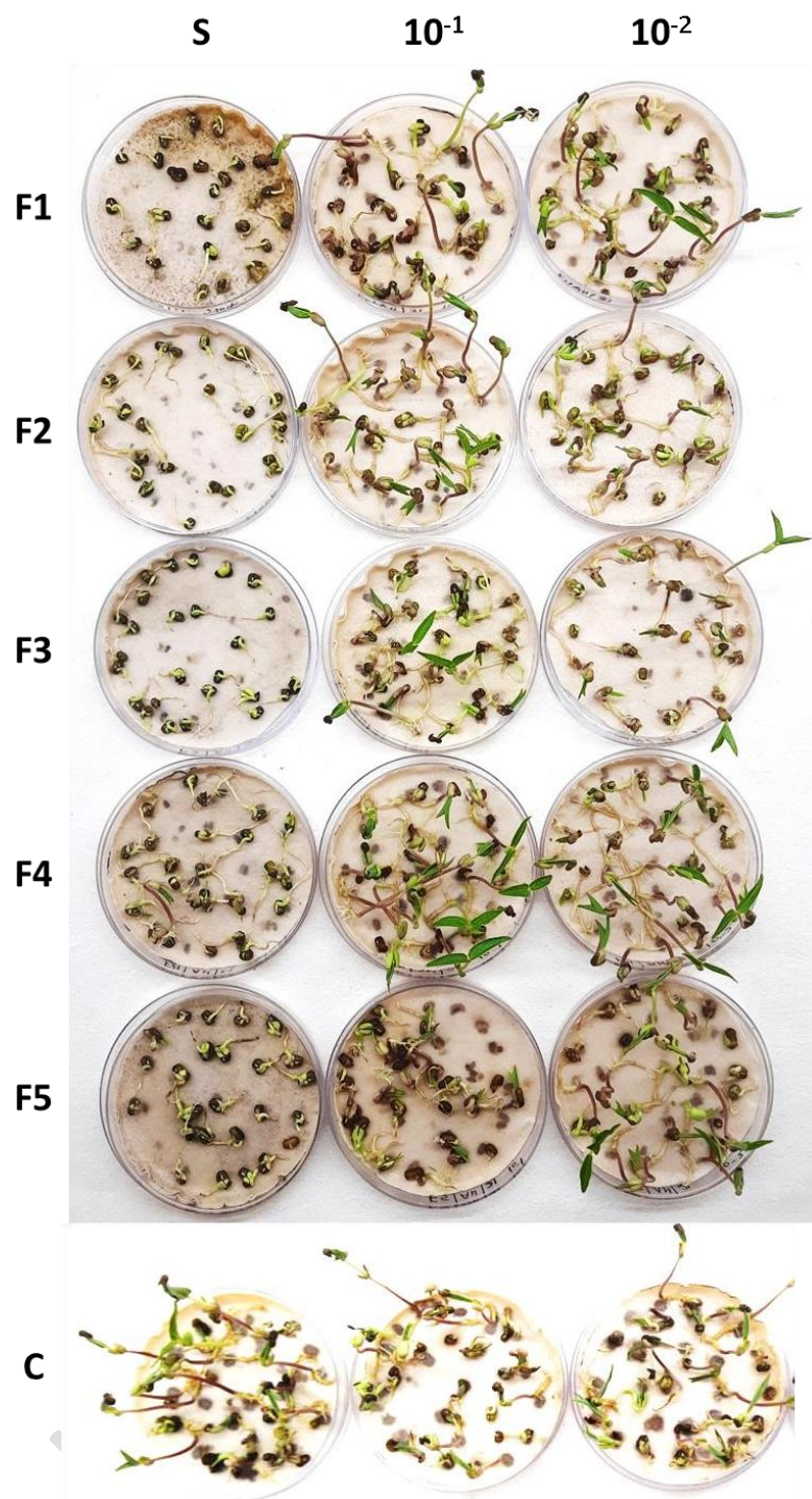
Figure 6: Phytotoxicity analysis of formulations 2 nd , 14 th and 21 st day on Greengram seedlings under aerobic and anaerobic conditions
