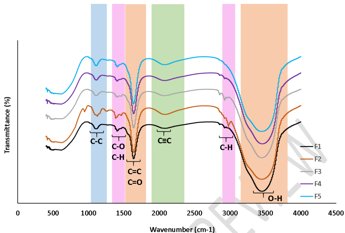
Figure 2: FTIR Analysis of different formulations
