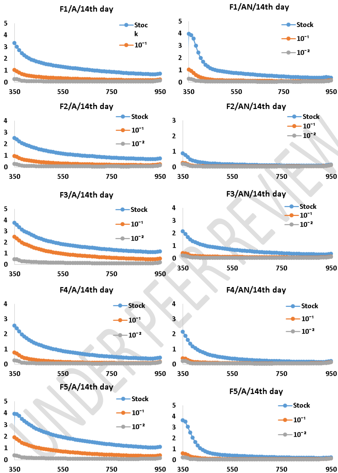
Figure 7: UV-Visible spectra of the formulations incubated for 14 days
