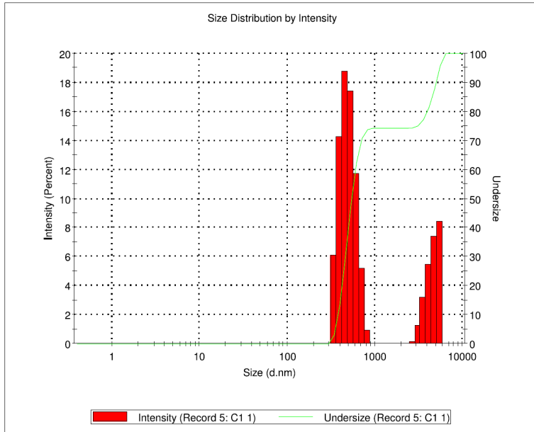
Figure 4: Particle size distribution in a tested formulation
