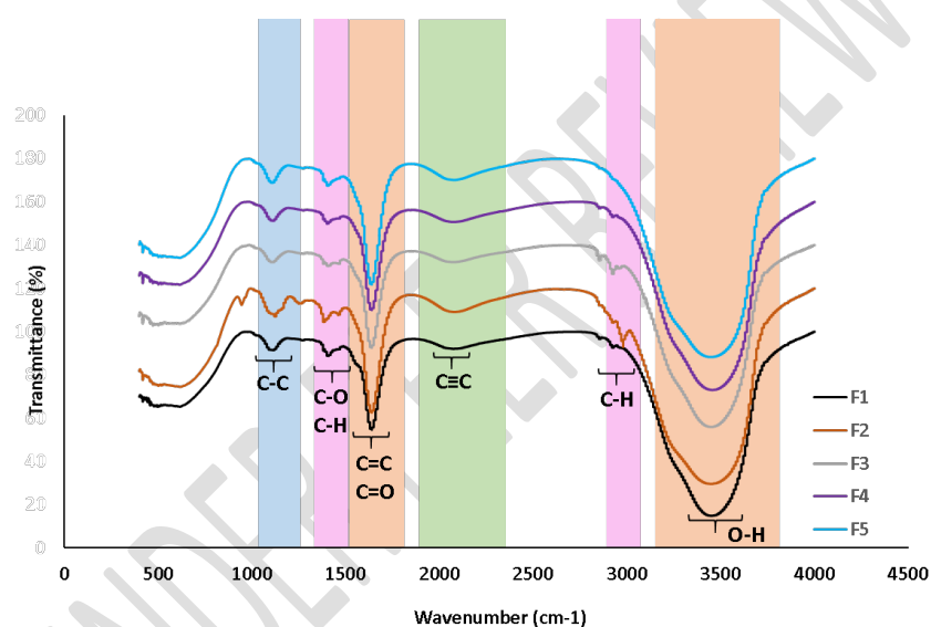
Figure 1: FTIR Analysis of different formulations
