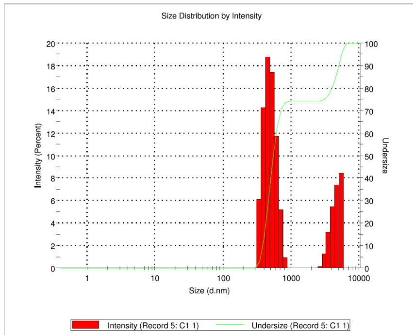
Figure 4: Particle size distribution in a tested formulation
