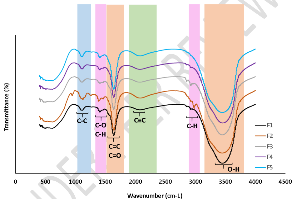
Figure 1: FTIR Analysis of different formulations
