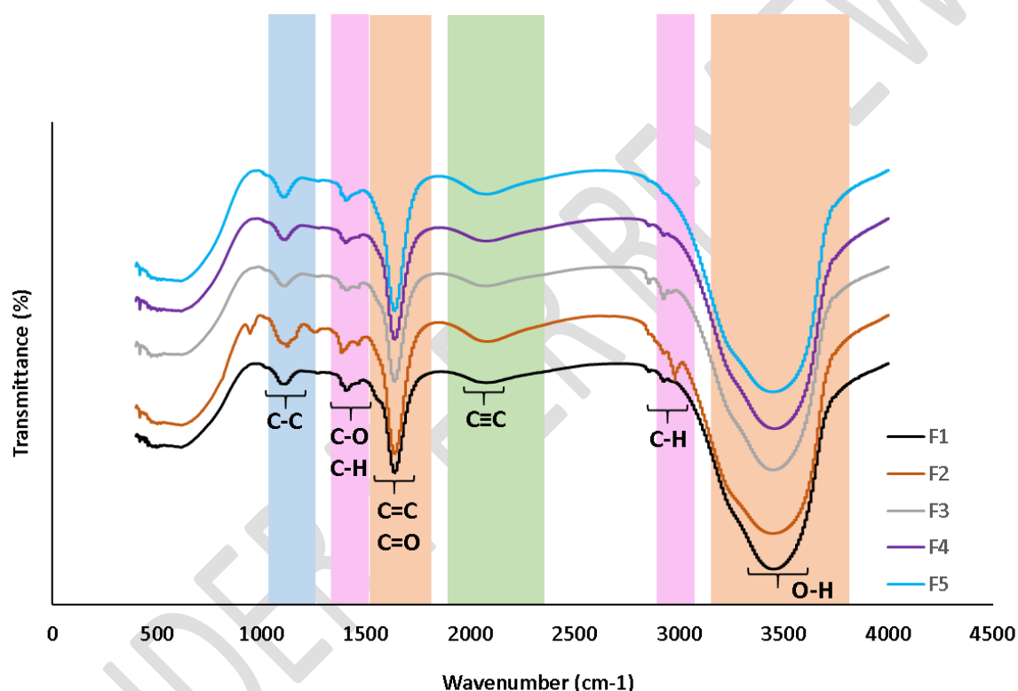
Figure 1: FTIR Analysis of different formulations
