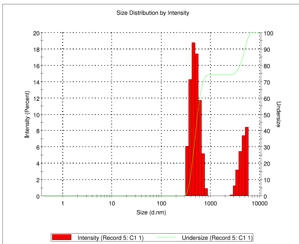
Figure 4: Particle size distribution in a tested formulation
