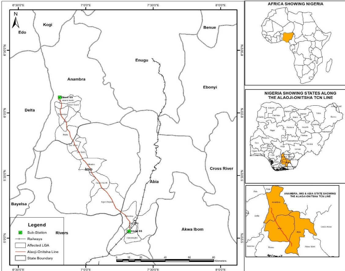
LOCATION MAP OF 330 kV ALAOJI-ONITSHA TRANSMISSION LINE
