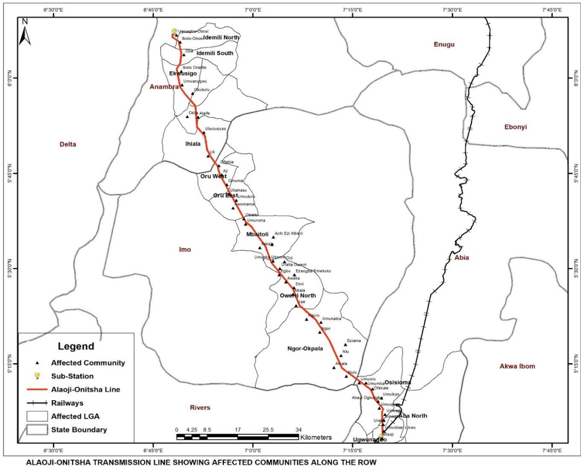
Figure 1: Map of the Transmission line route showing some communities and LGAs traversed within the three states
