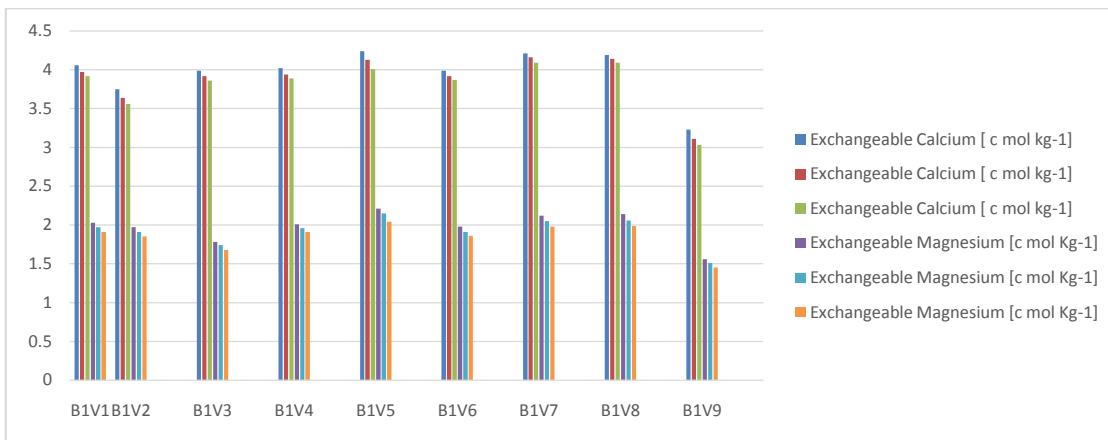
Fig4: Exchangeable Calcium and Magnesium [cmolKg -1 ]
