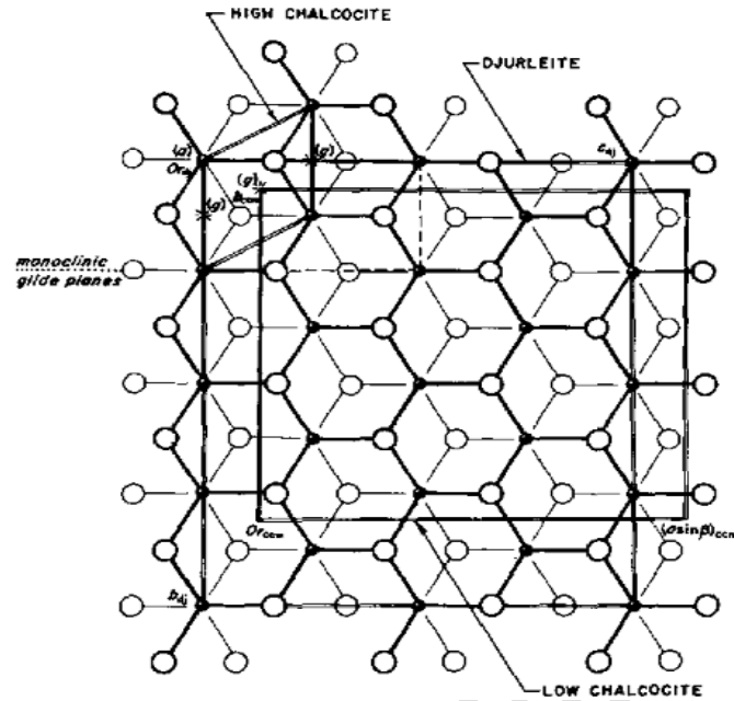
Fig. 1. Distribution scheme of copper and sulfur atoms in the phase lattice
