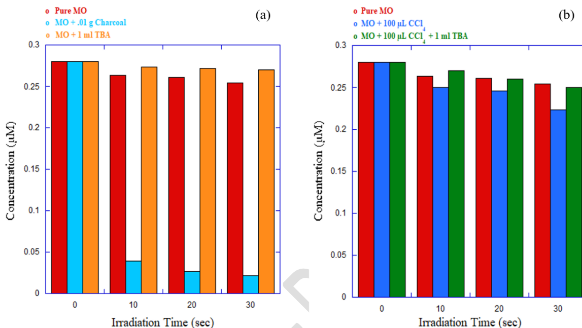
Figure 7: Microwave degradation of MO in the presence of TBA, CCl 4 , and charcoal, (a) TBA and Charcoal as an additive, (b) TBA + CCl 4 as an additive
