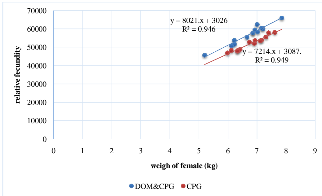
Figure 3: The correlation between the weight of females of grass carp and the relative fecundity (number of eggs/kg of body Wight) when treated with DOM and CPG and when treated with CPG alone.
