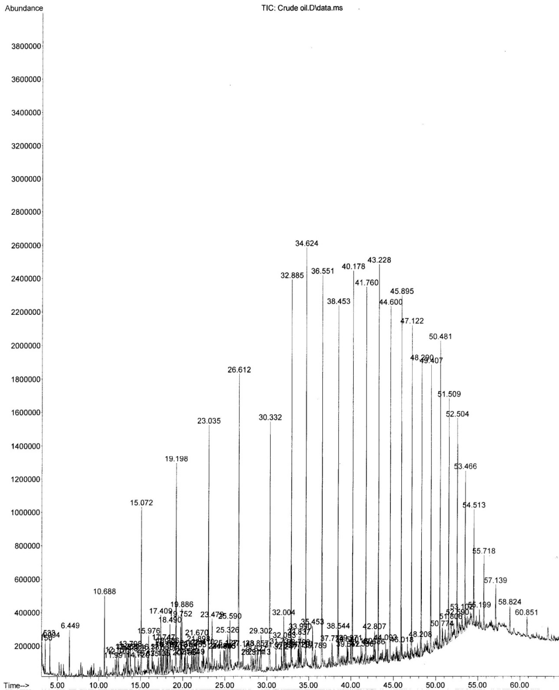
Fig. 5 : GC-MS Chromatograph of crude oil at zero time: (clear file attached)
