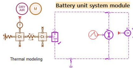
Figure 2. Simulation model of a single battery
