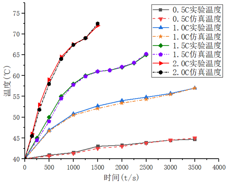
(c) Temperature comparison between simulation and experimental batteries at different discharge rates at 40°C
