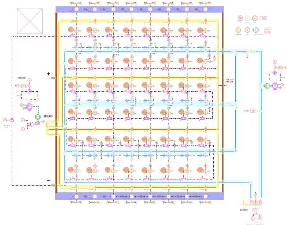
Figure 6. shows the thermal management model of battery opposite-direction composite refrigeration based on logic control
