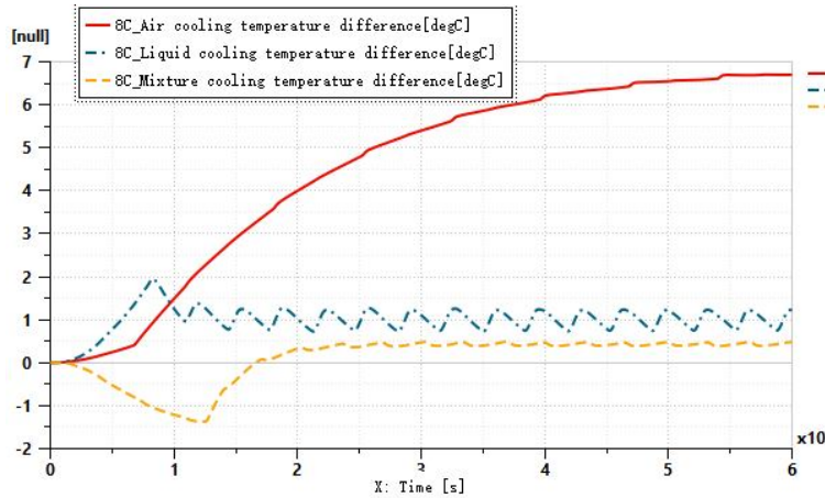
Figure 13. Curves of battery temperature differences under different cooling methods
