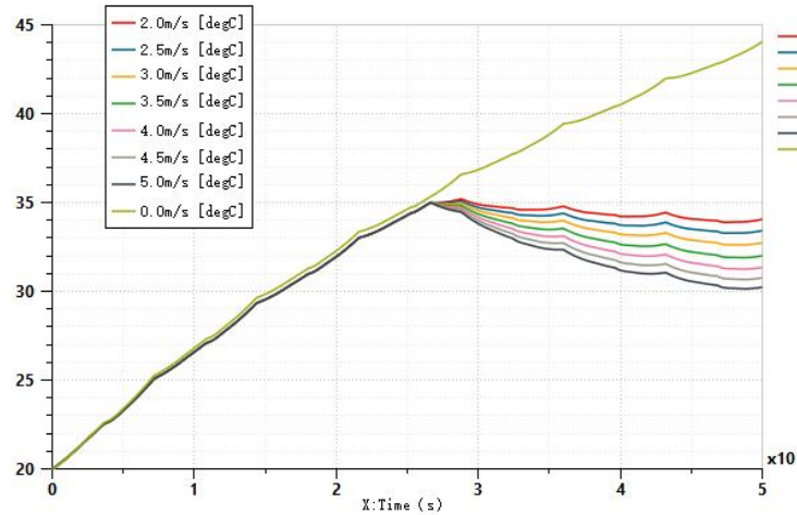
Figure 7. shows the temperature curve of power battery under different wind speeds
