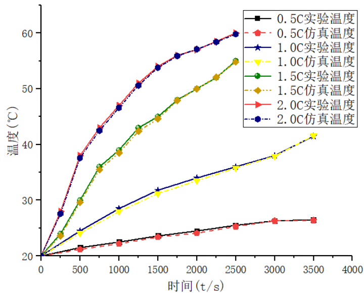
(a) Temperature comparison between simulation and experimental batteries at different discharge rates at 20^{\circ}\text{C}
