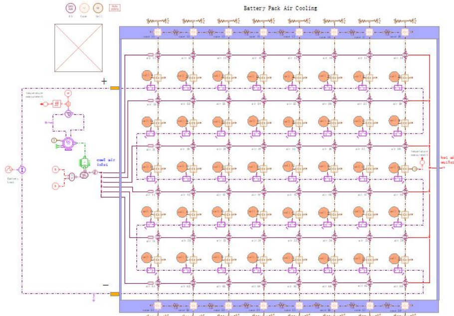
Figure 4. shows the battery air-cooled refrigeration model based on logic control
