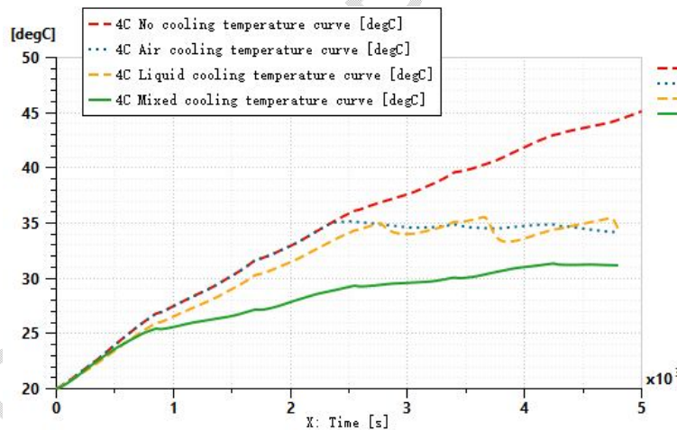
Figure 9. Temperature curves of thermal management of three kinds of batteries at 4 times charge-discharge ratios
