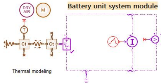
Figure 2. Simulation model of a single battery
