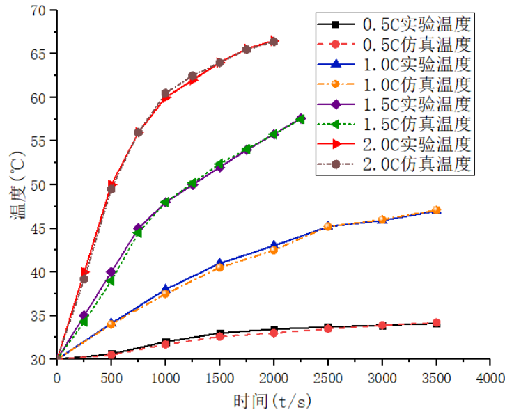
(b) Comparison of temperature between simulated and experimental batteries at different discharge rates at 30°C
