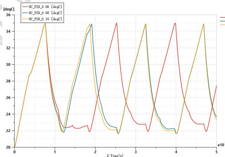
Figure 8. Curves of liquid cooling temperature under different mass flow rates
