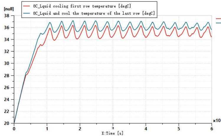
(b) Inlet and outlet temperature of liquid-cooled refrigeration batteries
