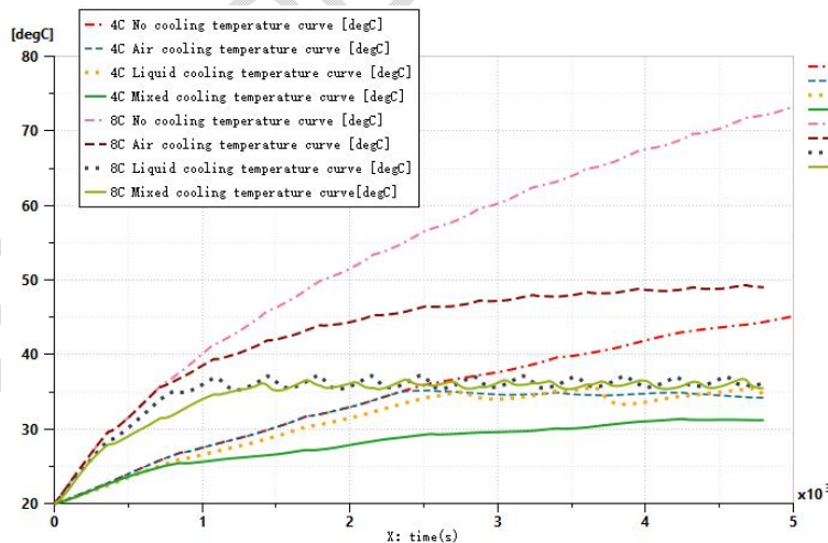
Figure 11. shows the temperature change curves of the three schemes under different charging and discharging ratios
