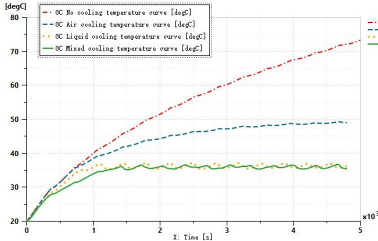
Figure 10. Thermal management temperature curves of three kinds of batteries at 8 times charge-discharge ratio
