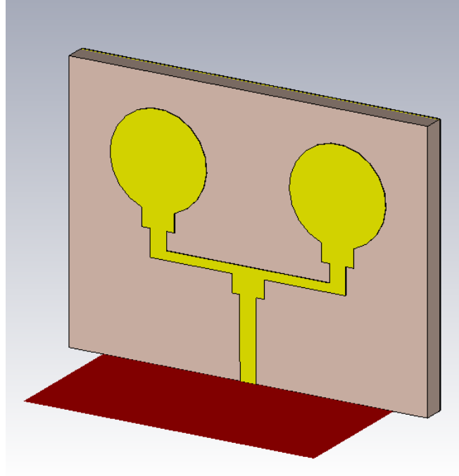
Fig. 2. 1 \times 2 Circular Array Antenna Perspective View
