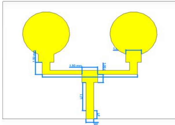
Fig. 1. 1 × 2 Circular Array Antenna Dimensions
