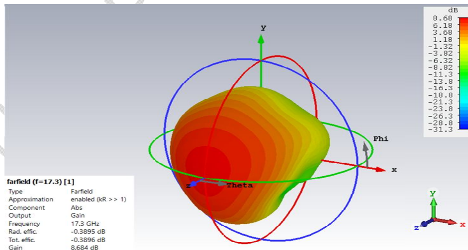
Fig. 5. Antenna Gain
