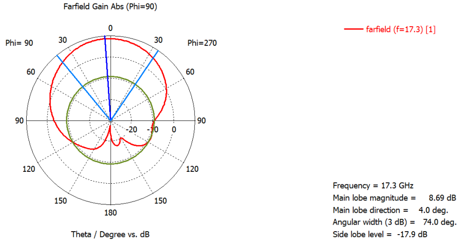
Fig. 6. Antenna Gain in Planar view
