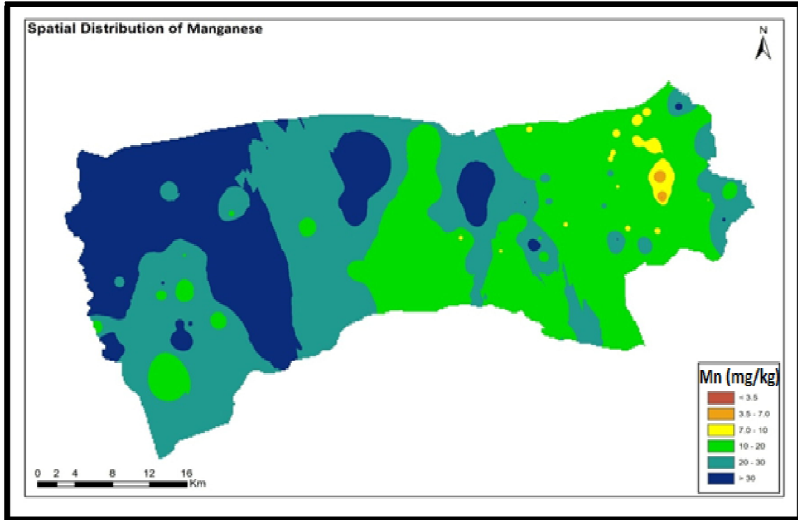
Fig. 16. Spatial distribution of DTPA-Mn (mg/kg) in the soils of Biswanath district (Assam)
