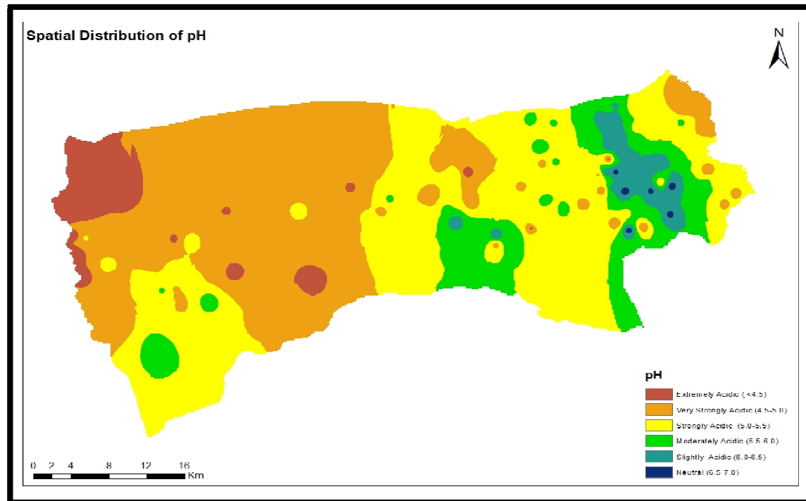
Fig. 2. Spatial distribution of pH in the soils of Biswanath district (Assam)
