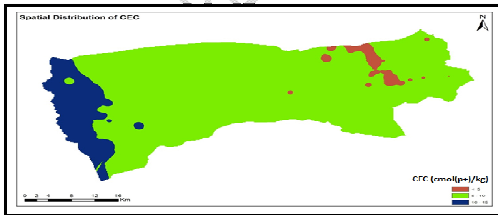
Fig. 4. Spatial distribution of cation exchange capacity ( \text{cmol}(\text{p}+)/\text{kg} ) in the soils of Biswanath District, Assam
