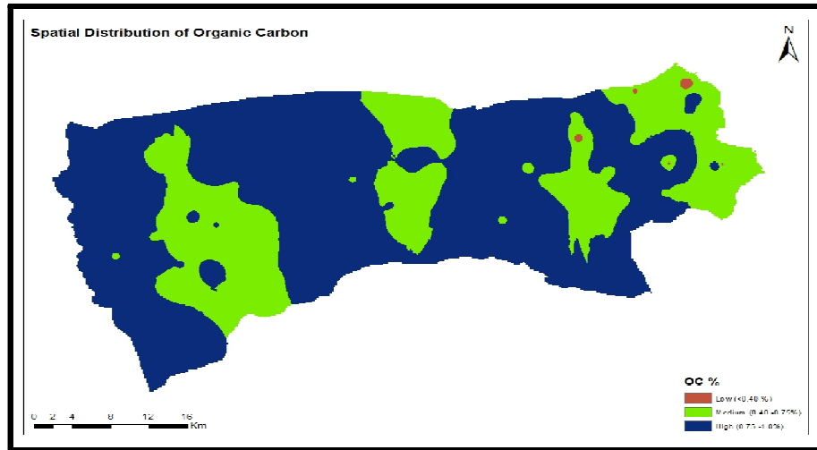
Fig. 3. Spatial distribution of organic carbon per cent in the soils of Biswanath of Biswanath District, Assam
