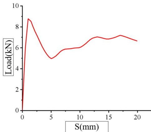
Fig. 3 .Load-Slip Curve
