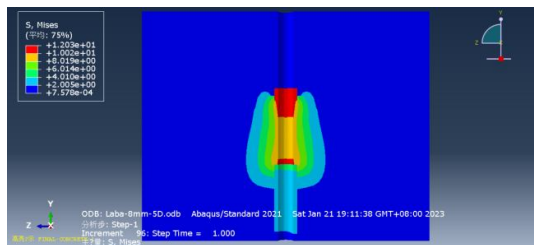
Fig.9. Concrete Stress Cloud Diagram
