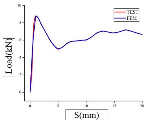
Fig.10. Comparison Of Test And Finite Element Results
