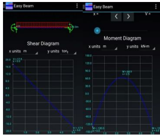
Fig. 8. output internal force]
