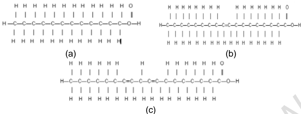
Figure 3. Fish Oil Chemical Structure: (a) SFA, (b) MUFA, (c) PUFA Source: Sartika[21]
