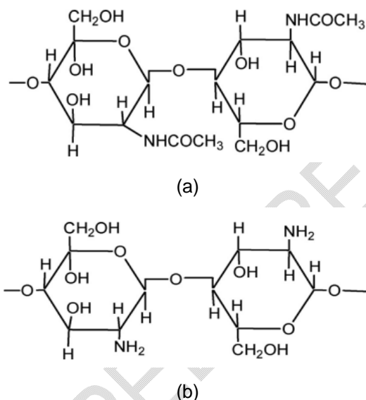
Figure 2. Chemical Structure of Chitin and Chitosan (a) Chitin (b) Chitosan Source: Hassan et al. [16]
