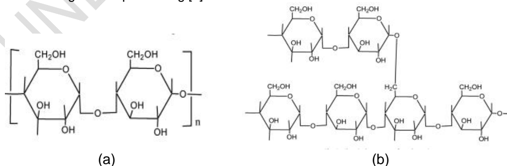
Figure1. Starch Ingredients Chemical Structure (a) Amylose (b) Amylopectin. Source: Hassan et al. [16]
