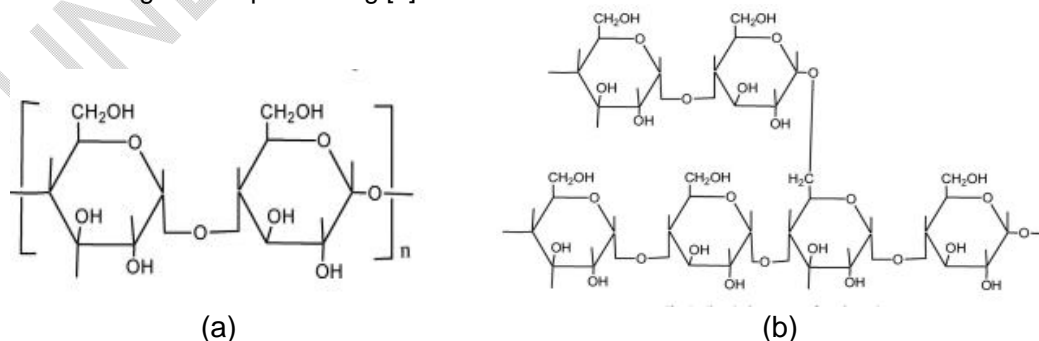
Figure 1. Starch Ingredients Chemical Structure (a) Amylose (b) Amylopectin.
