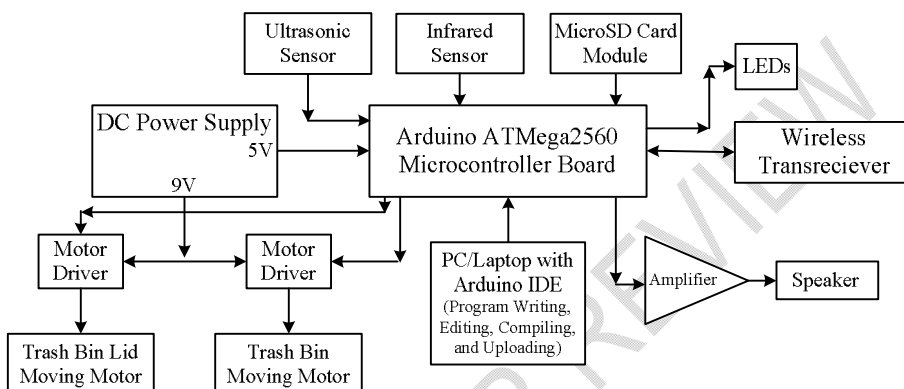
Fig. 1. Block diagram of the whole diagram
