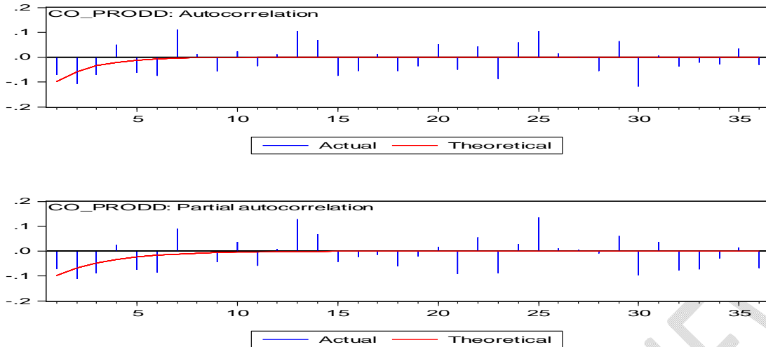
Figure 6: Graphs of the ACF and PACF respectively, for Crude Oil Production
