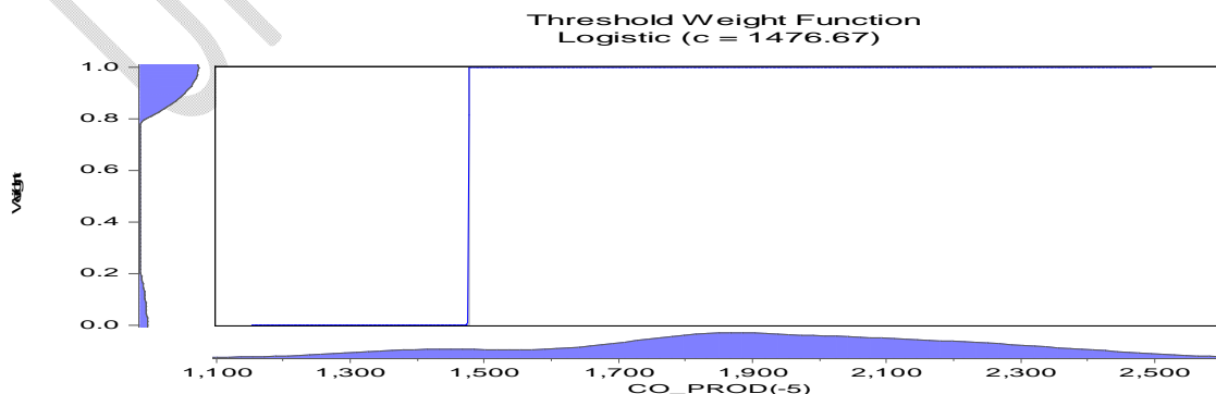
Figure 7: Graph Threshold Smoothing Weight
