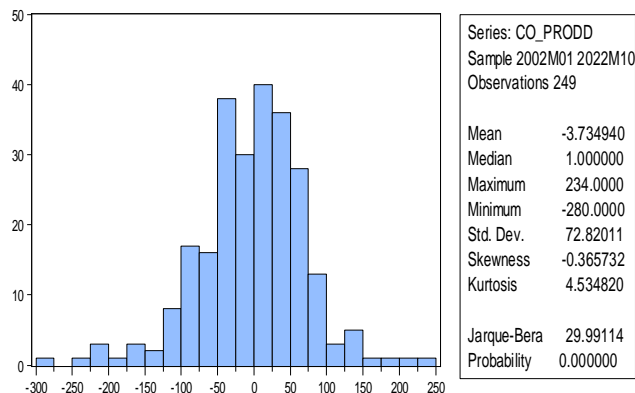
Fig. 5: Histogram of the Differenced Data
