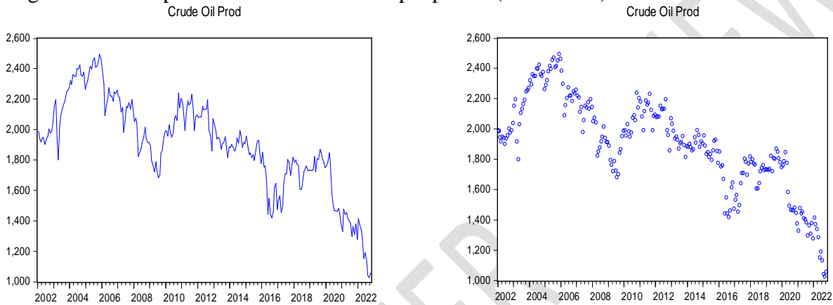
Fig. 1: Time Plot of Crude Oil Production
