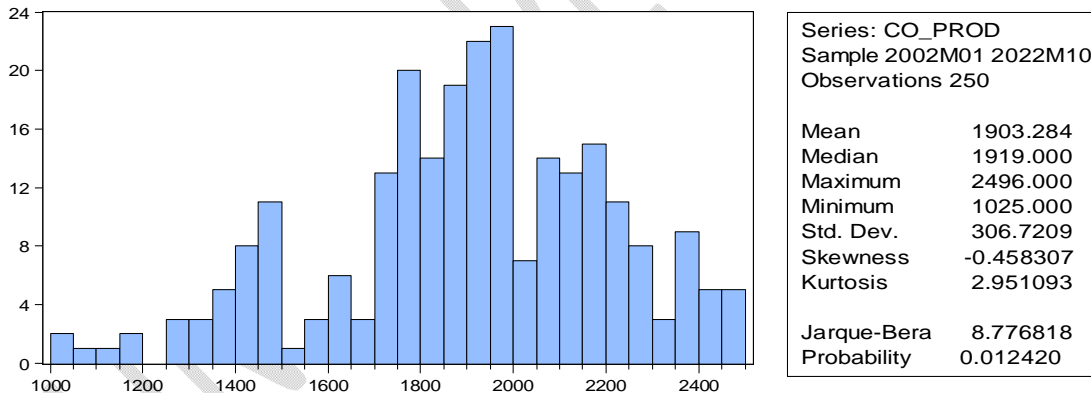
Fig. 3: Histogram of the Crude Oil Productions
