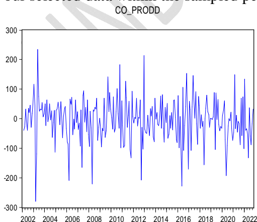
Fig. 4: Time plot of Differenced Data
