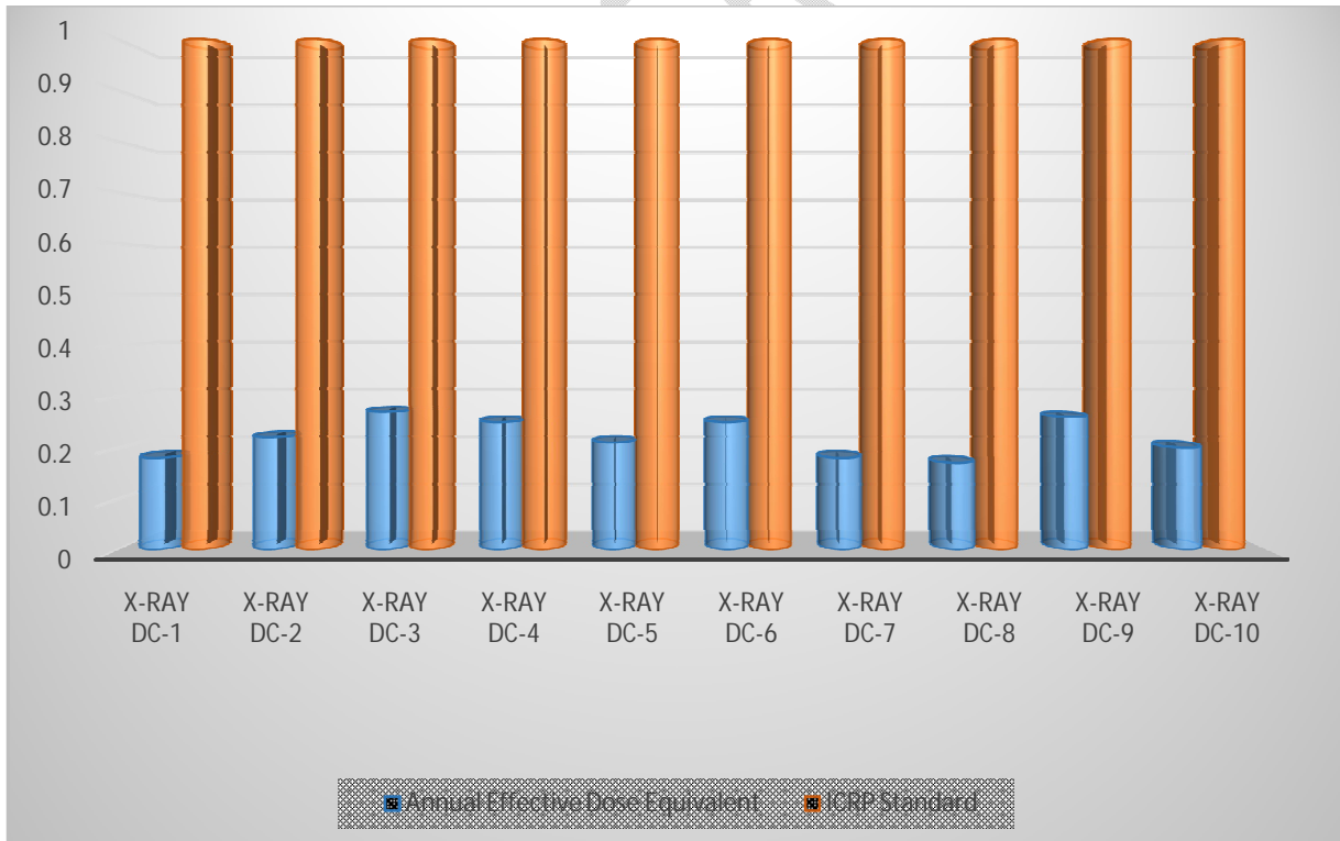
Figure 3. Chart of Annual Effective Dose Equivalent of the sampled X-ray diagnostic centers
