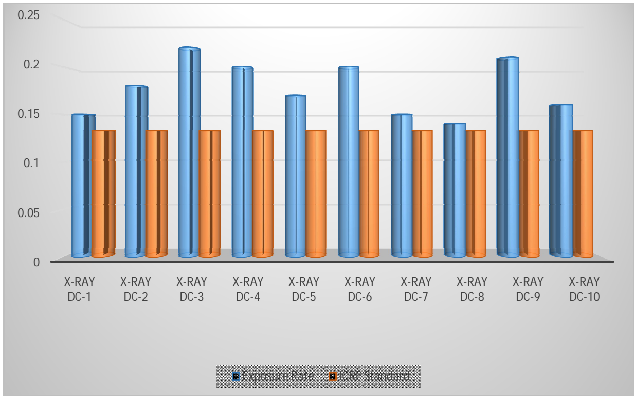
Figure 2. Chart of exposure rate of the sampled X-ray diagnostic centers
