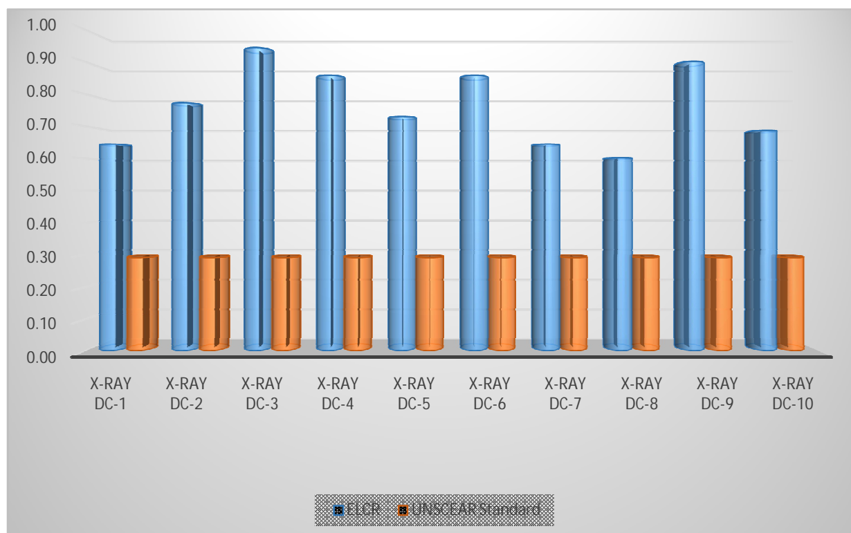
Figure 4. Chart of Excess Lifetime Cancer Risk of the sampled X-ray diagnostic centers
