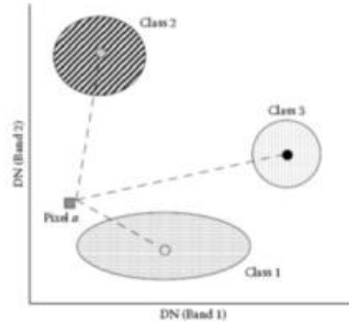
Figure3: Schematic visualization of the minimum distance from the mean classifier [13]
