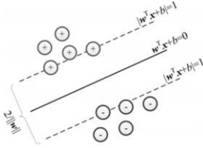
Figure7: A view of binary linear SV [14]
