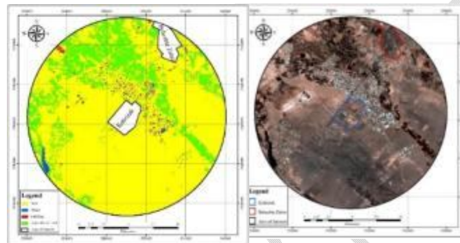
Figure26: VCI index
