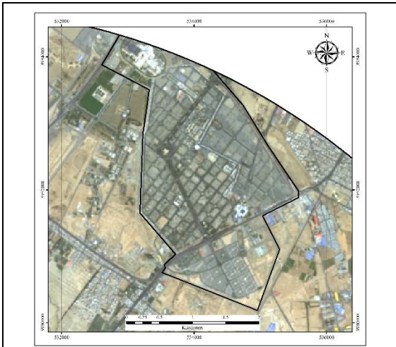
2017-09-11 Landsat8 image
