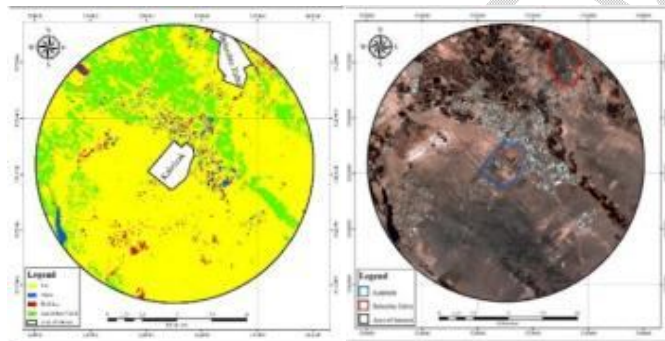
Figure23: LAI index
