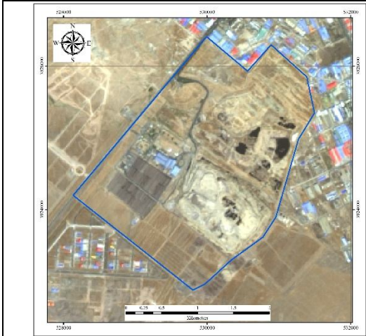
2020-09-19 Landsat8 image
