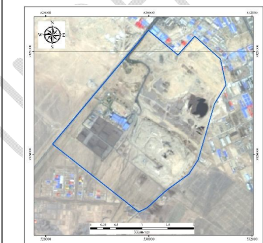
2015-09-06 Landsat8 image
