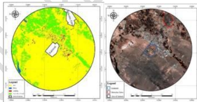
Figure24: SAVI index
