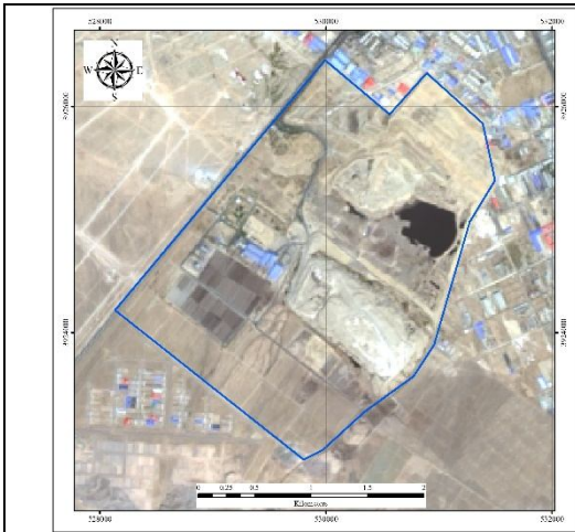
2013-09-16 Landsat8 image
