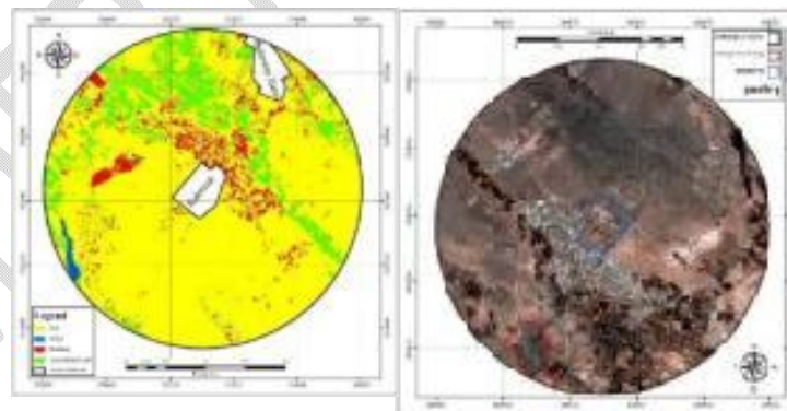
Figure18: Support vector machine classification with circular kernel
