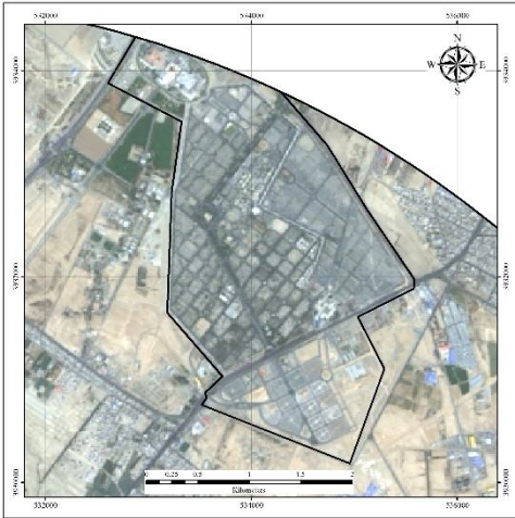
2014-09-19 Landsat8 image
