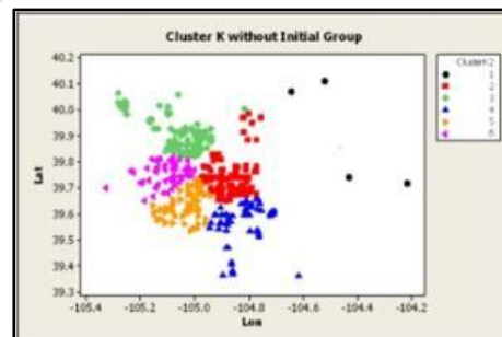
Figure 10: k-means category [13]
