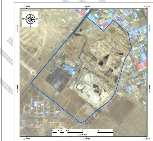
2021-09-22 Landsat8 image
