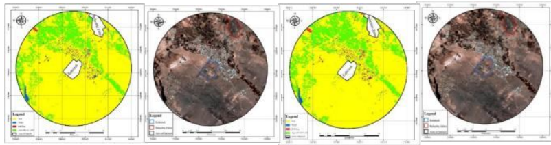
Figure26: VCI index
