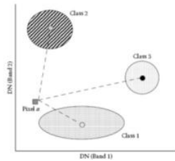
Figure3:Schematic visualization of the minimum distance from the mean classifier (Alavi Panah, 2013)
