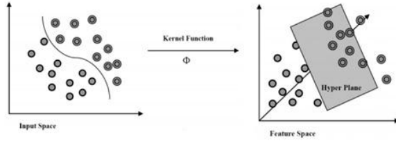
Figure 8: Nonlinear separation using fan kernel SVMs (Borges, 1998)
